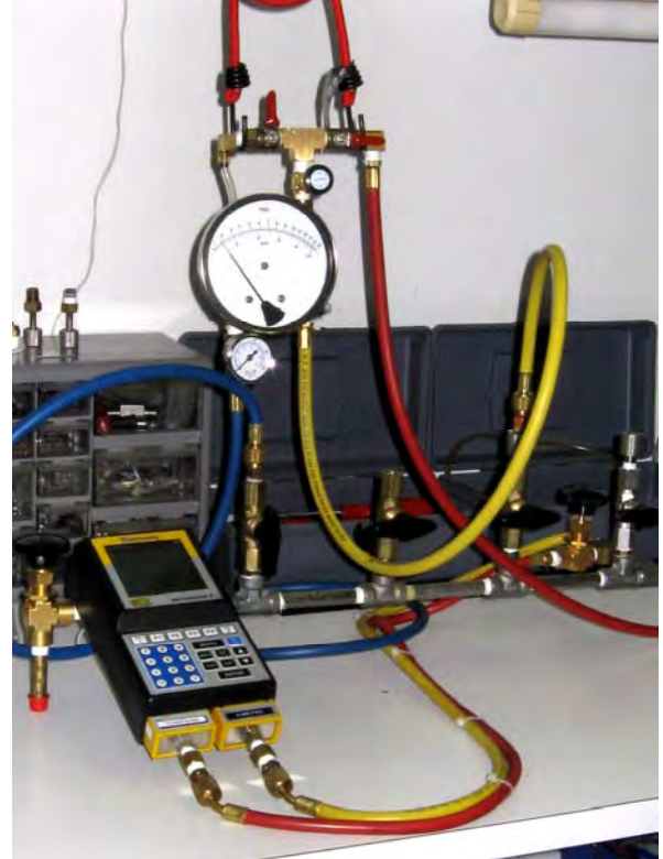
A backflow kit being certified in BBI's state of the art calibration lab
